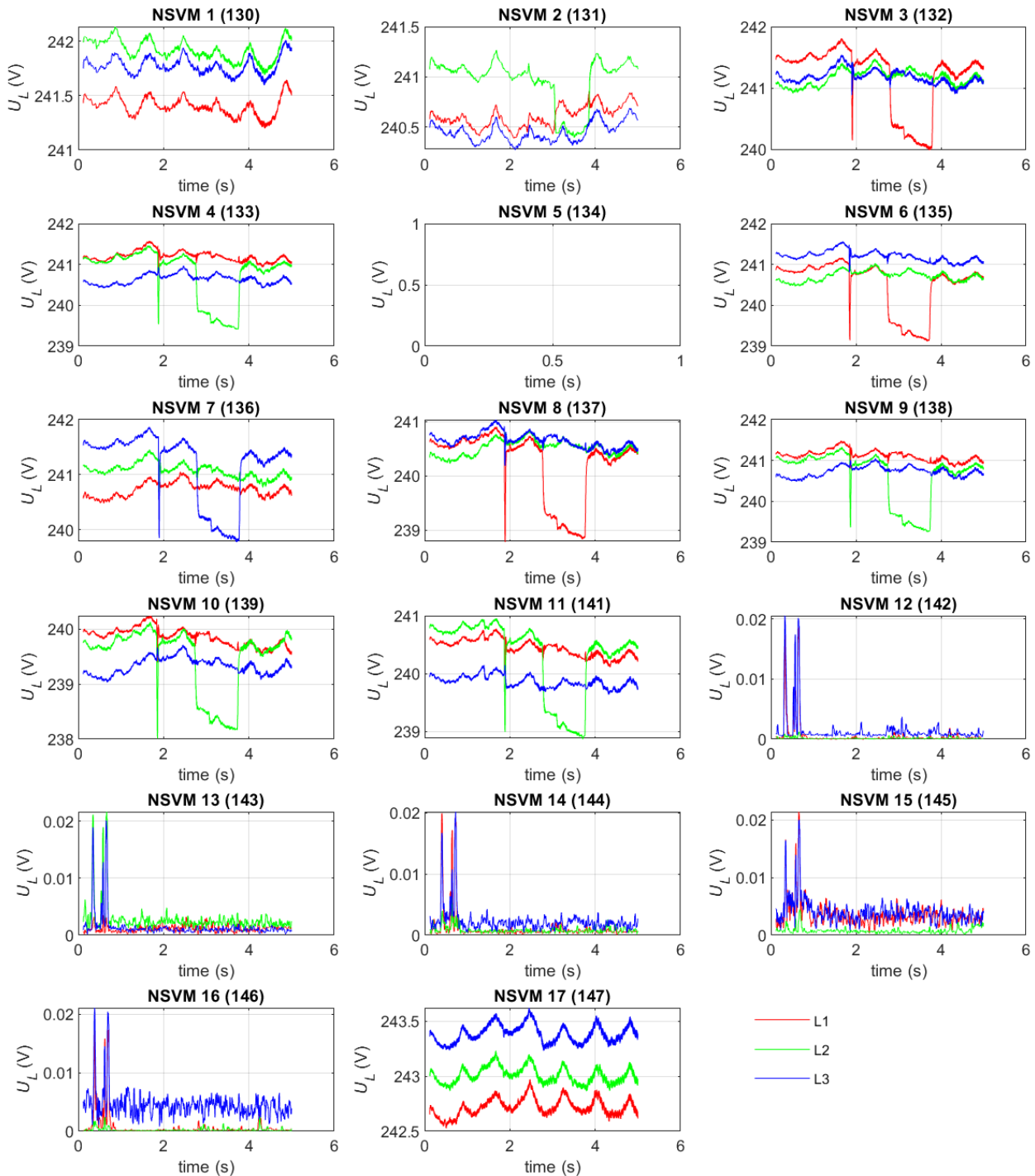
Fig. 6: RMS value of phase voltages recorded by DMUs during fault No. 13
