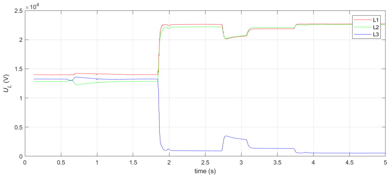
Fig. 1: RMS value of phase voltages recorded by feeder protection during fault No. 13
