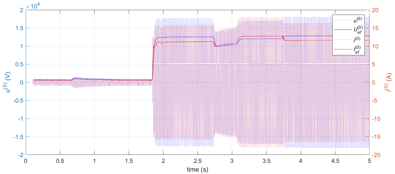
Fig.3: Zero sequence currents and voltages recorded by feeder protection during fault No. 13
