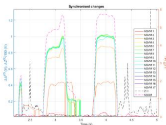
Fig. 7: Negative sequence current and voltage changes of NSCM and NSVM recorded during fault No. 13
