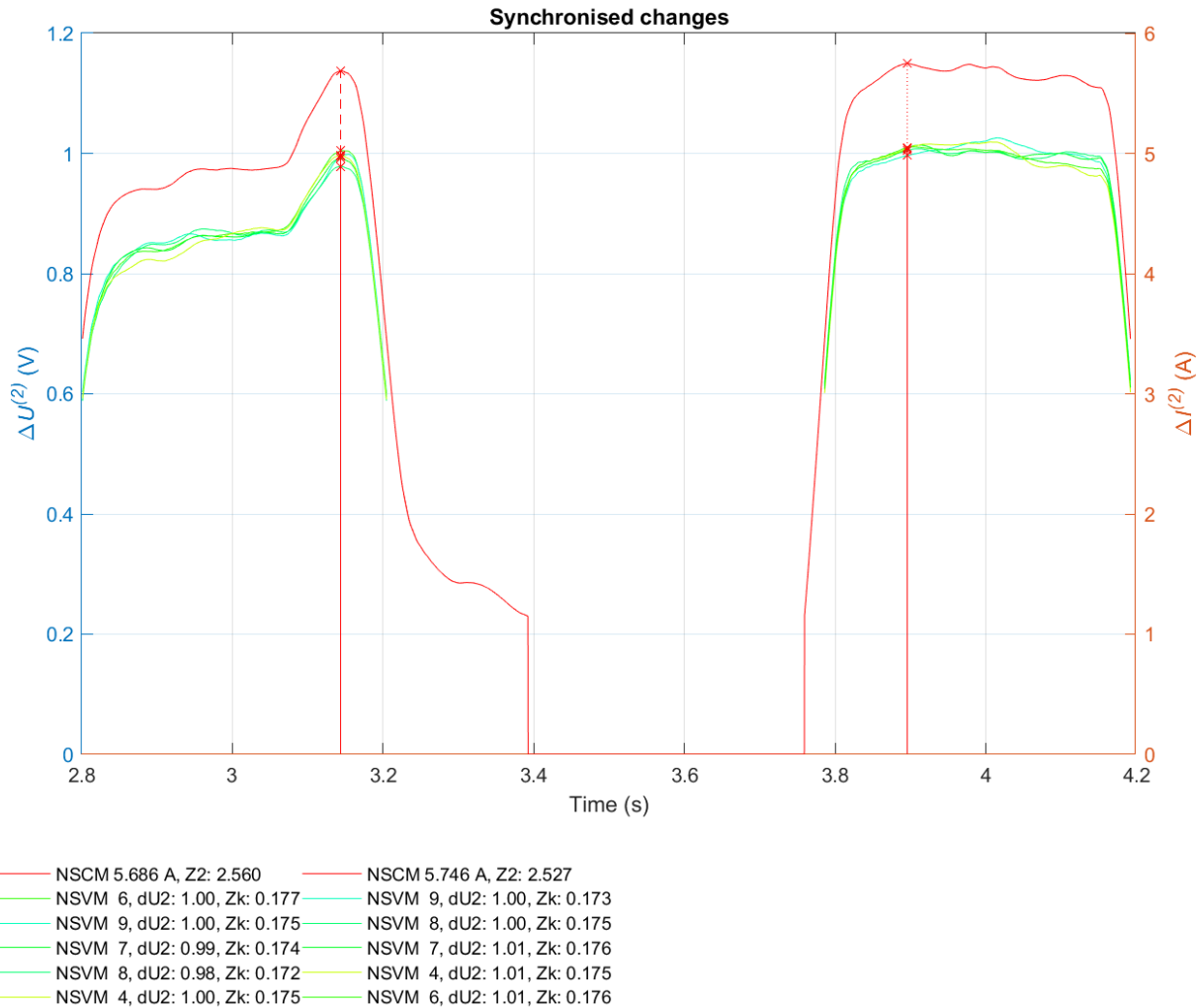
Fig. 8: Negative sequence current and voltage changes for individual synchronization pulses of fault No. 13
