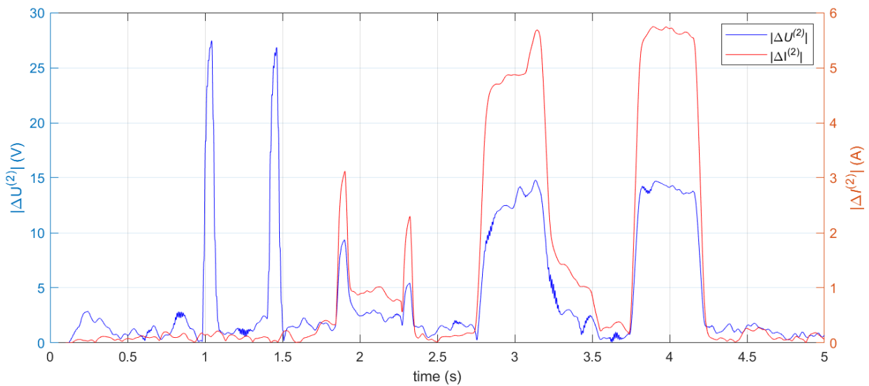
Fig. 5: Change in negative sequence current and voltage recorded by feeder protection (NSCM) during fault No. 13
