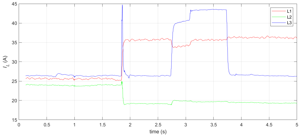
Fig. 2: RMS value of phase currents recorded by feeder protection during fault No. 13
