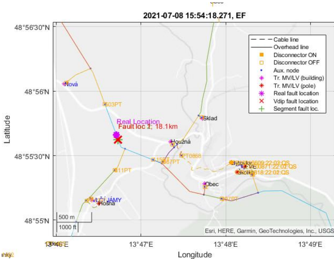
Fig. 9: Presentation of fault location estimated by Vdip method for data of fault record No. 13.
