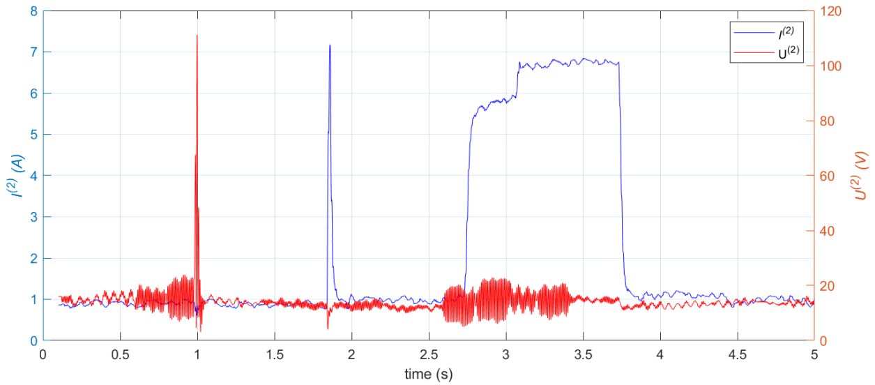
Fig. 4: Negative sequence current and voltage magnitudes recorded by feeder protection during fault No. 13
